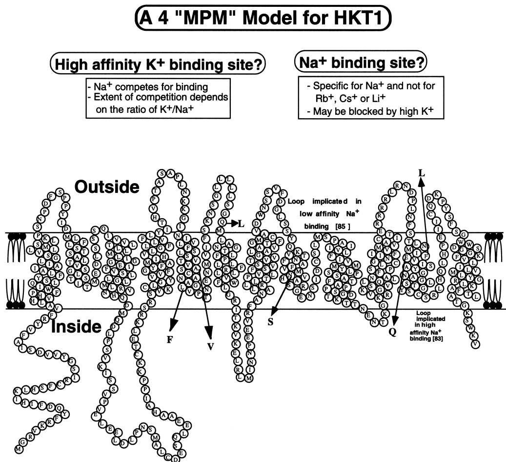
Fig. 3. A topological model of HKT1 based on the consensus of five membrane transporter predication programs and a recently proposed model [81]. The functional features that were proposed by [71] and the mutations that alter functional characteristics are highlighted [72,83,85].
